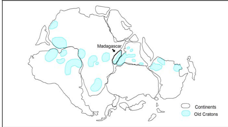
Figure Dia-1: Map of Gondwana showing the location of ancient cratonic cores.
